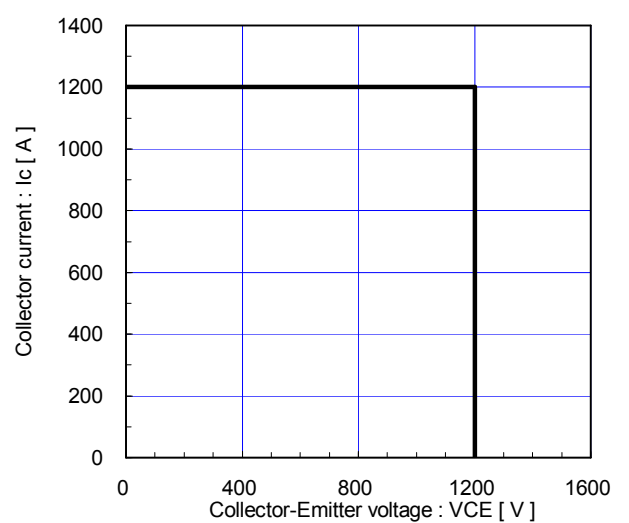
Reverse bias safe operating area (max.) +V_{GE}=15V, -V_{GE} \le 15V, R_G \ge 0.6\Omega, T_J \le 125^\circ C
