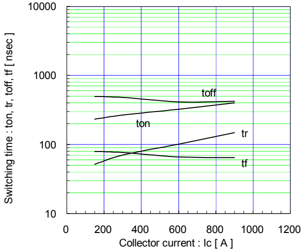
Switching time vs. Collector current (typ.) V_{CC}=600V, V_{GE}=\pm 15V, R_G=0.6\Omega, T_J=25^\circ C
