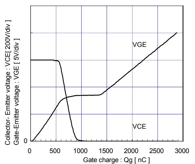
Dynamic Gate charge (typ.) Vcc=600V, Ic=600A, Tj=25°C
