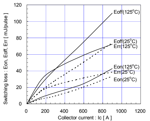
Switching loss vs. Collector current (typ.) V_{CC}=600V, V_{GE}=\pm 15V, R_G=0.6\Omega
