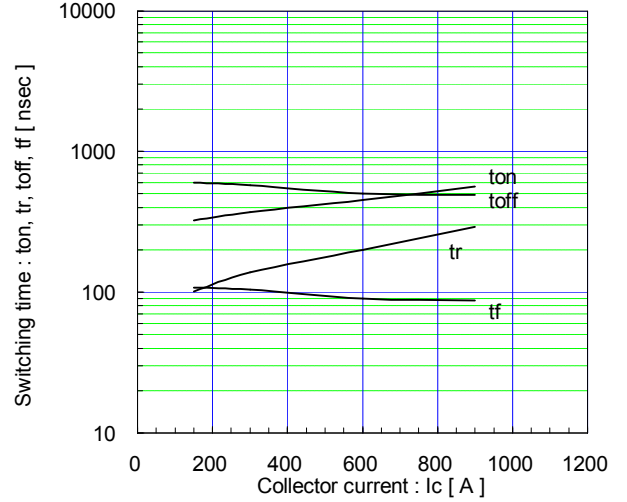
Switching time vs. Collector current (typ.) V_{CC}=600V, V_{GE}=\pm 15V, R_G=0.6\Omega, T_J=125^\circ C
