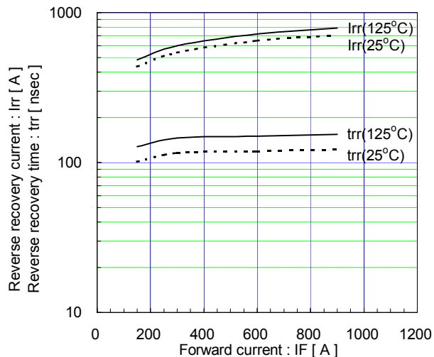
Reverse recovery characteristics (typ.) Vcc=600V, VGE=±15V, RG=0.6Ω
